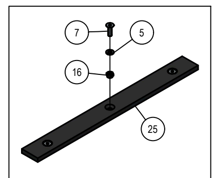
Detail C
